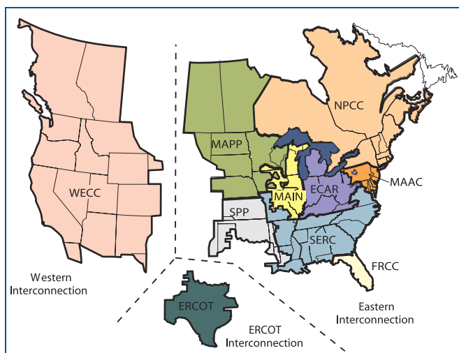
Figure 2.2. NERC Interconnections
